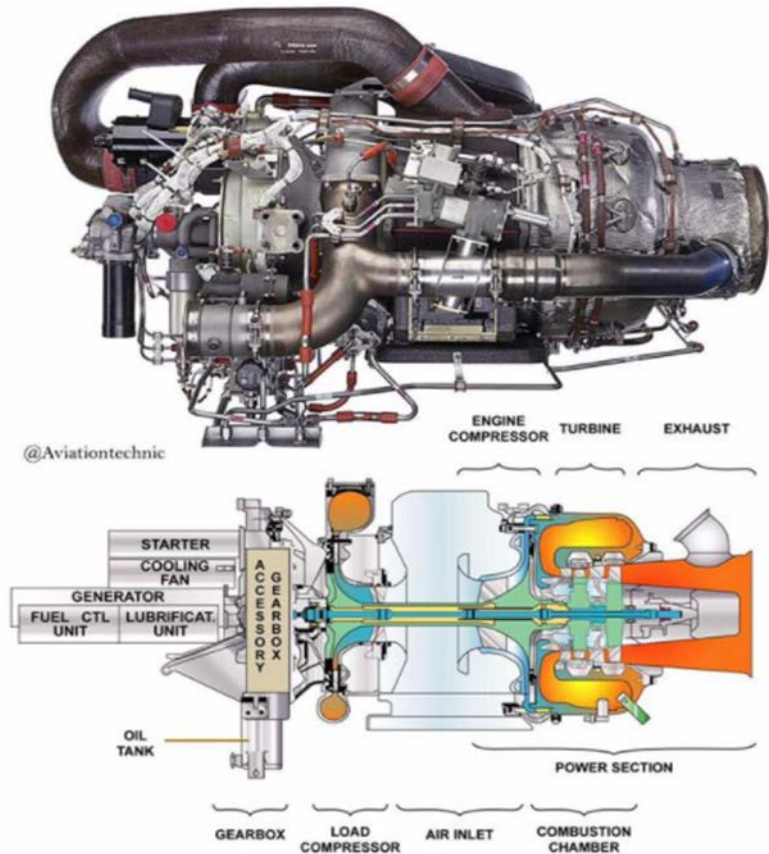
Auxiliary Power Unit (APU)
